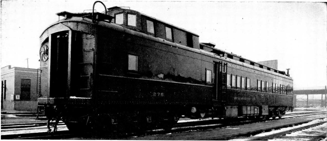
Fig. 874—Northern Pacific All-Steel Dynamometer Car Built at Como Shops, St. Paul, Minn., Weight 168,000 lb.; Capacity for Drawbar Pull of 250,000 lb. and Buffing Shock of 1,250,000 lb.
