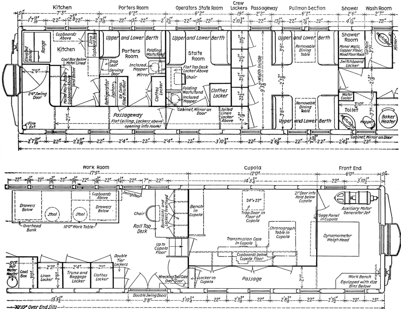
Fig. 875—Floor Plan of Northern Pacific Dynamometer Car Showing Arrangement of Accommodations and Apparatus.
